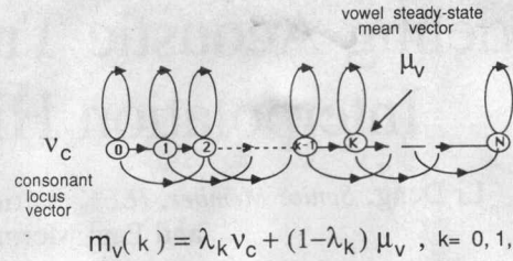
Fig. 1. A vowel HMM having an acoustic transition structure. The left-most K states (labeled 0 to K-1 ) represent the consonant-to-vowel transition. The state labeled K (shown) and a few states to the right of it (omitted for clarity) represent the vowel's stationary portion. The remaining states represent the vowel-to-consonant transition (omitted also).
